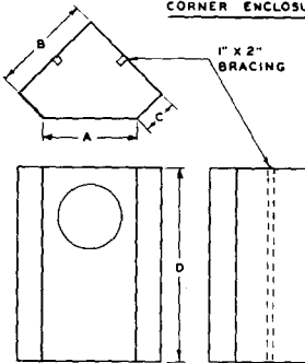
CORNER ENCLOSURES
